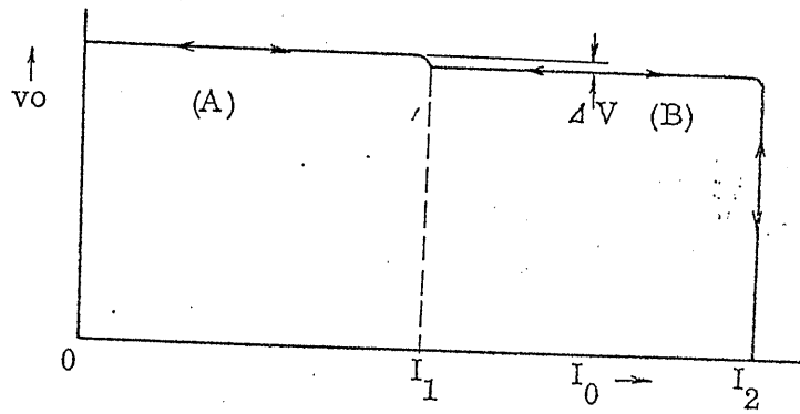
Fig. 3-9 Characteristics diagram
