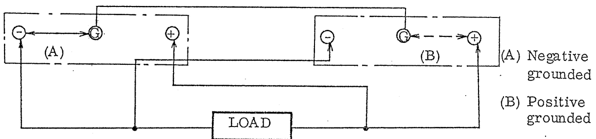
Fig. 3-8 Parallel connection diagram
