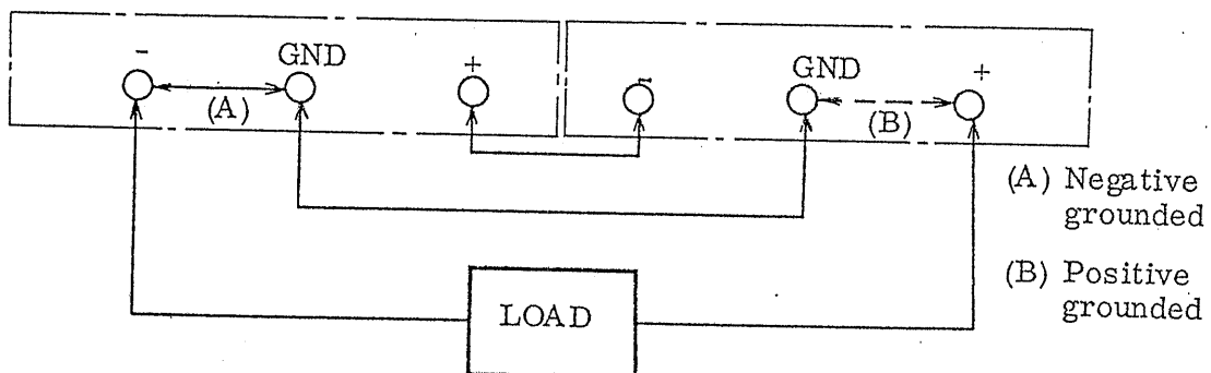
Fig. 3-5 Series connection diagram
