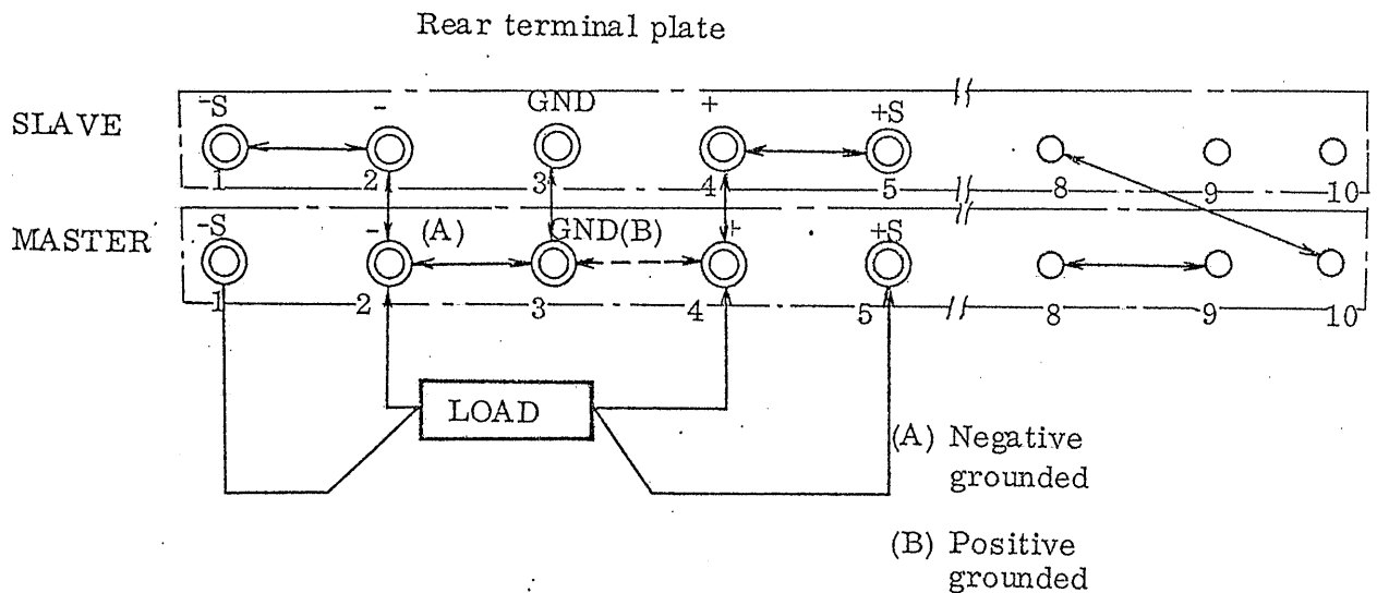
Fig. 3-11 Using sampling terminal in one-control parallel operation
